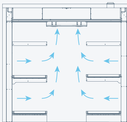
Horizontal Airflow
