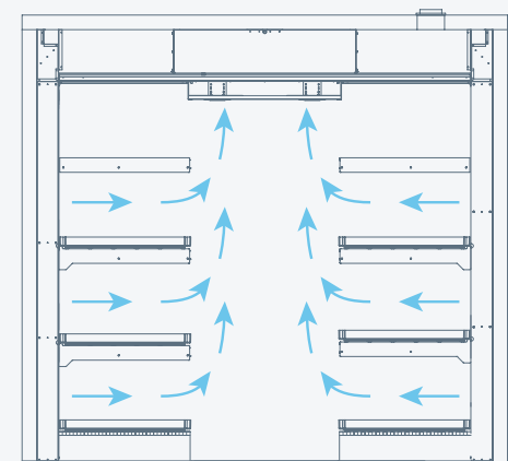
Horizontal Airflow
